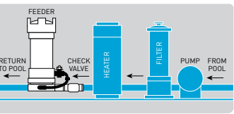
Illustration of Model 320 Feeder
