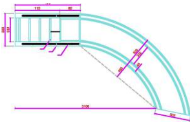
SLIDING BOARD TOP VIEW (RIGHT SIDE)
