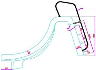
SLIDING BOARD LEFT SIDE VIEW
