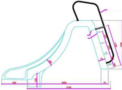
SLIDING BOARD LEFT SIDE VIEW
