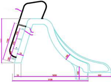
SLIDING BOARD RIGHT SIDE VIEW
