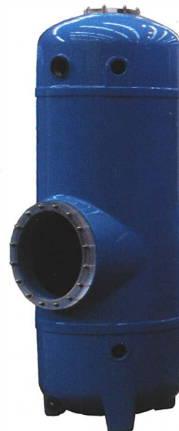
Threaded connections integrated in body Transparent top lid Access manhole Top diffuser Sight glass Nozzle plate Nozzle detail Drain plug
