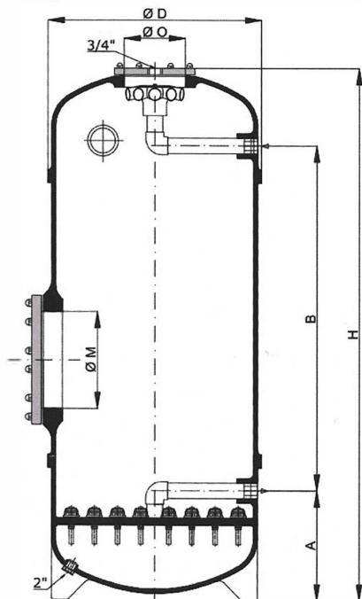
Threaded connections integrated in body Transparent top lid Access manhole Top diffuser Sight glass Nozzle plate Nozzle detail Drain plug
